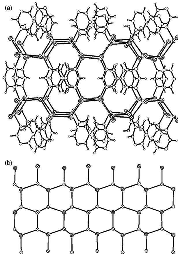
Fig. 4 Molecular structure of [\text{Cu}_2\text{I}_2(\text{tri})]_x : (a) view showing the alternating [\text{Cu}]_x and triazine layers and (b) view of the two-dimensional [\text{Cu}]_x layer (Cu, hatched; I, cross-hatched; N, dotted; C, shaded).
